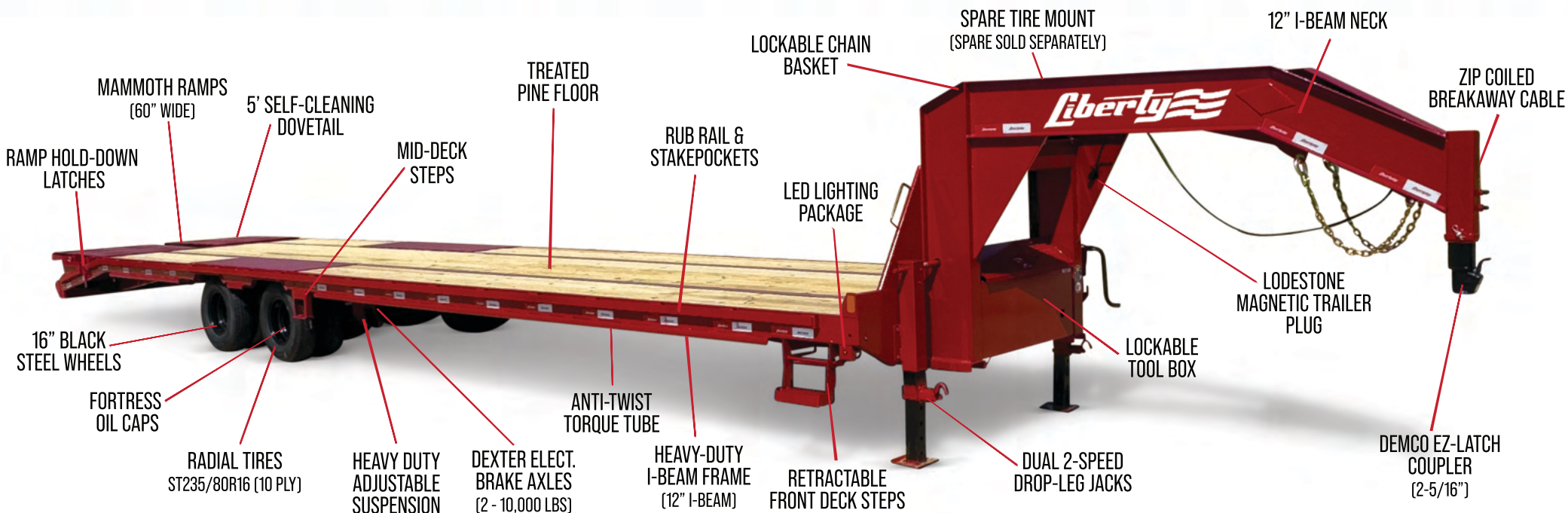
5' DOVETAIL & MAMMOTH RAMPS
