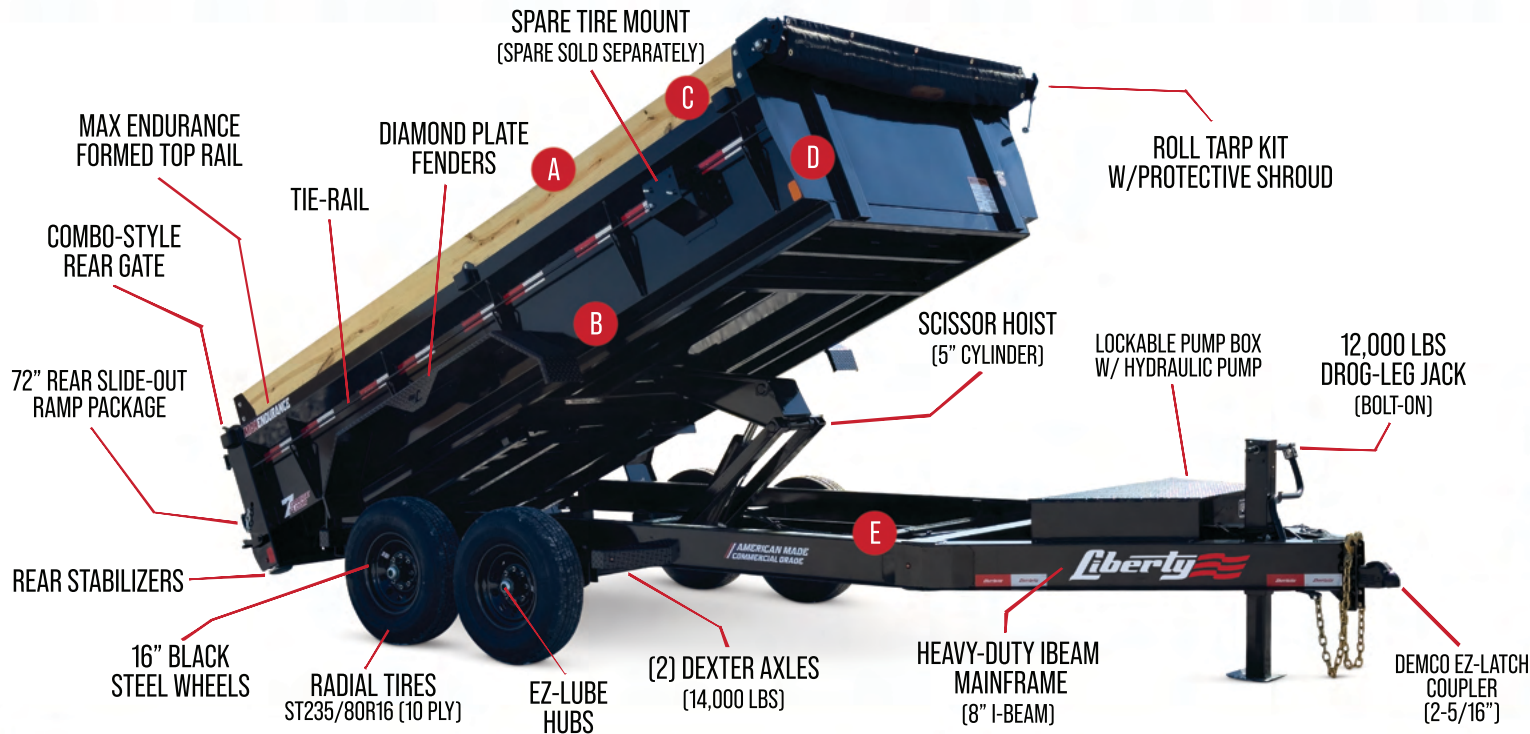
STURDY SCISSOR HOIST W/ 45° DUMP ANGLE
